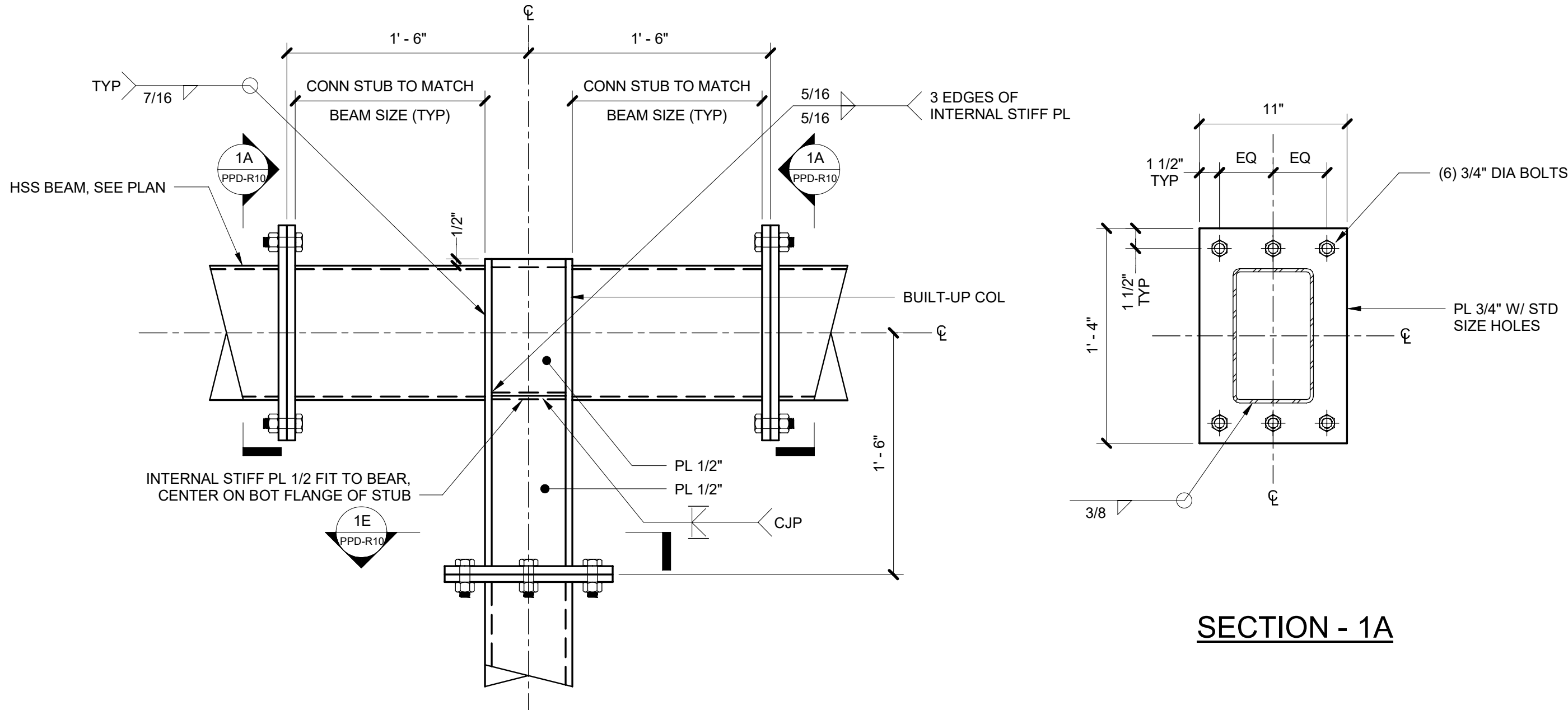
HSS10X6 BEAM/HSS6X6 COLUMN
