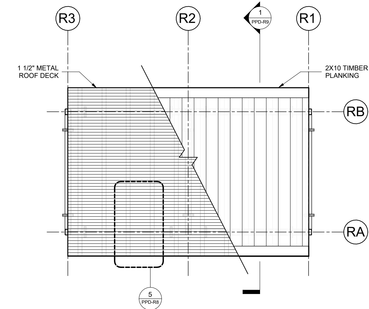
1 PART PLAN - DECK TYPE D1 1/4" = 1'-0"
