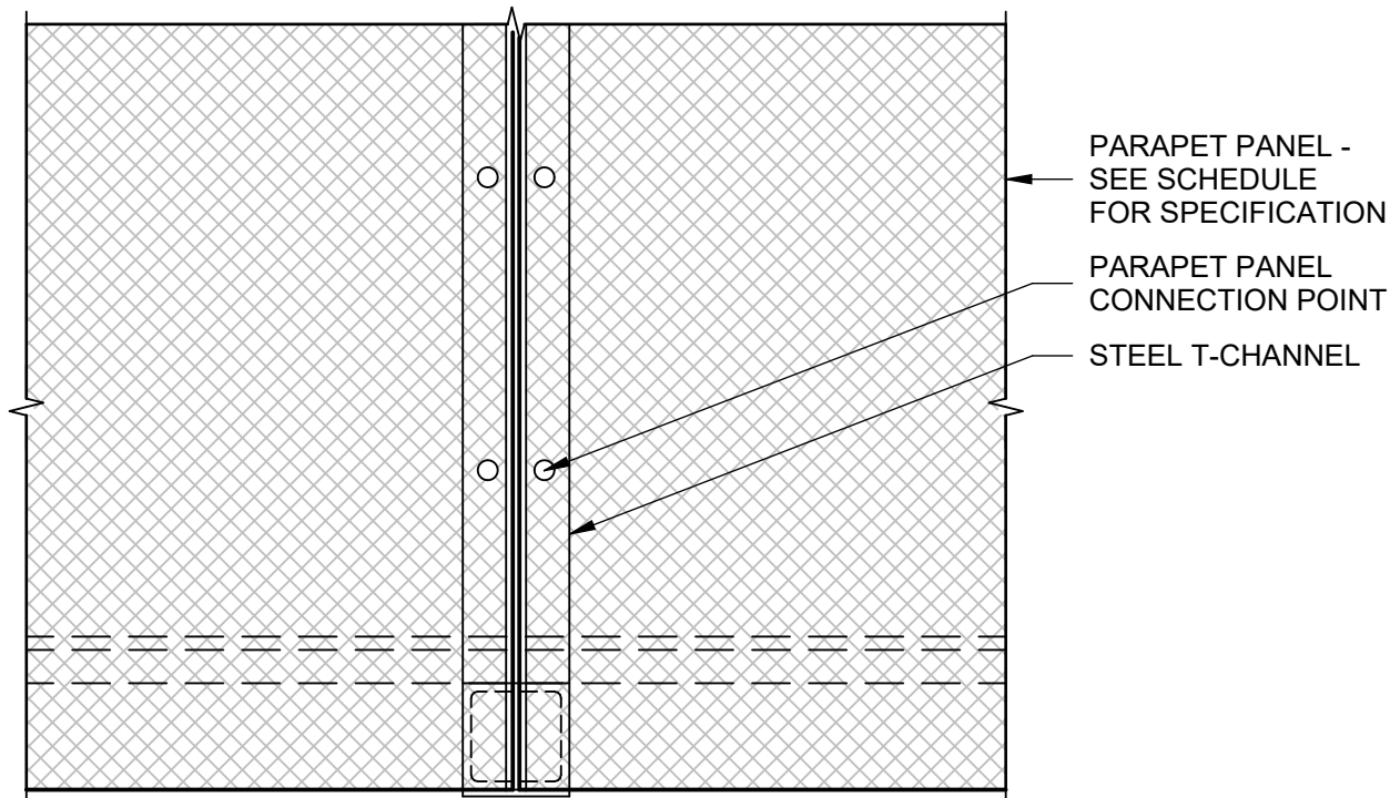
5 ELEVATION DETAIL 1 1/2" = 1'-0"
