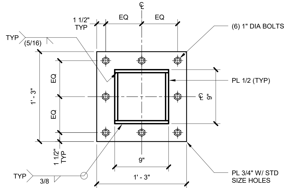
SECTION - 1F
