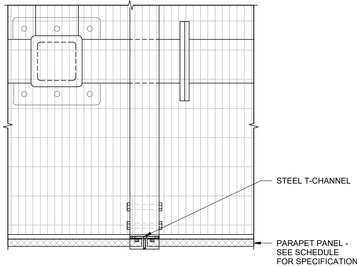
4 PLAN DETAIL 1 1/2" = 1'-0"
