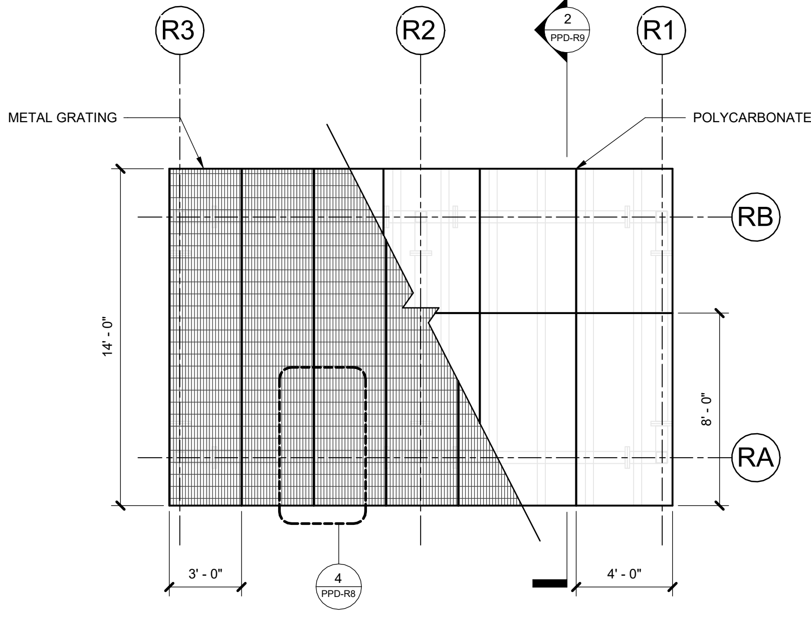
2 PART PLAN - DECK TYPE D2 1/4" = 1'-0"
