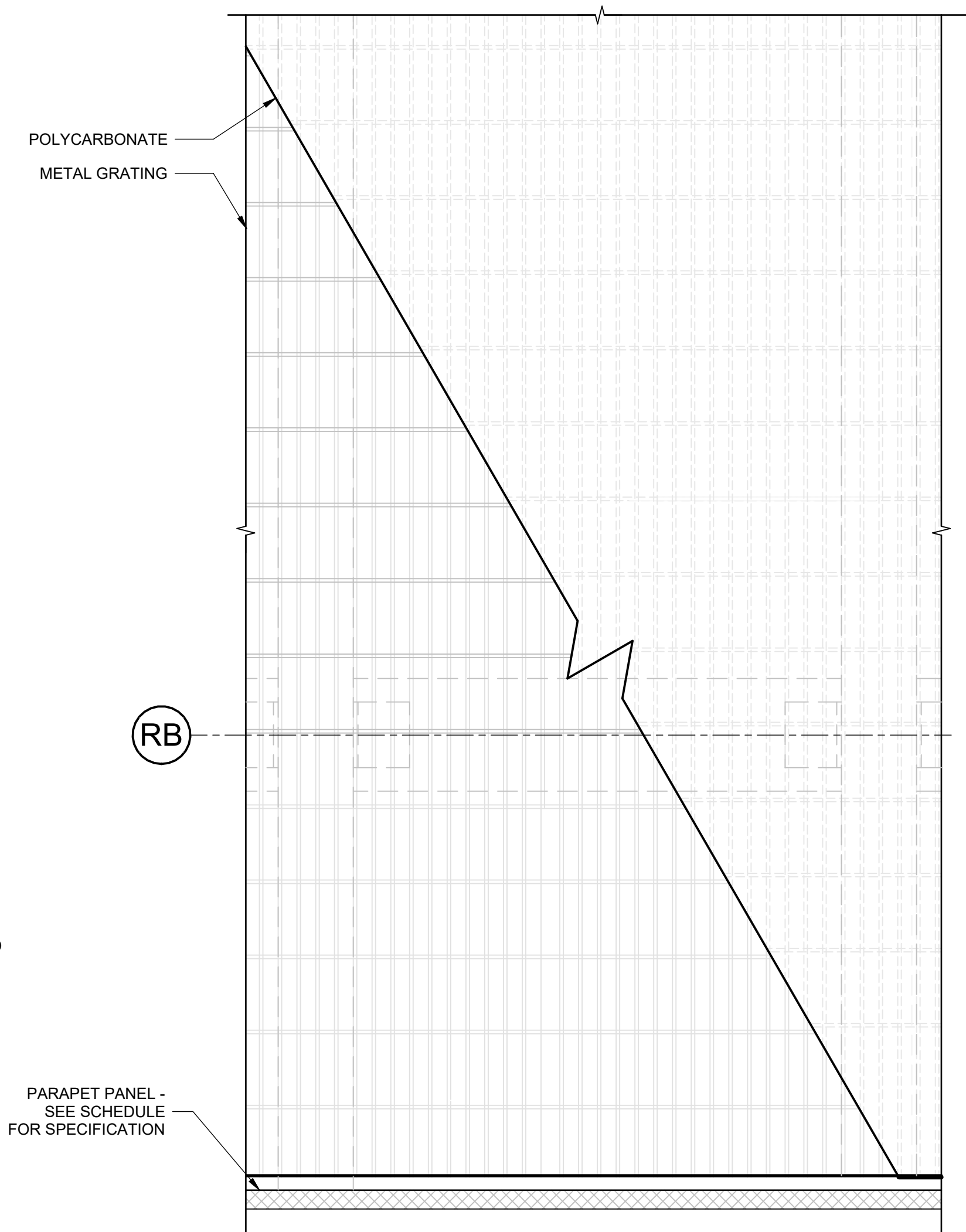
4 PLAN DETAIL - DECK TYPE D2 2" = 1'-0"
