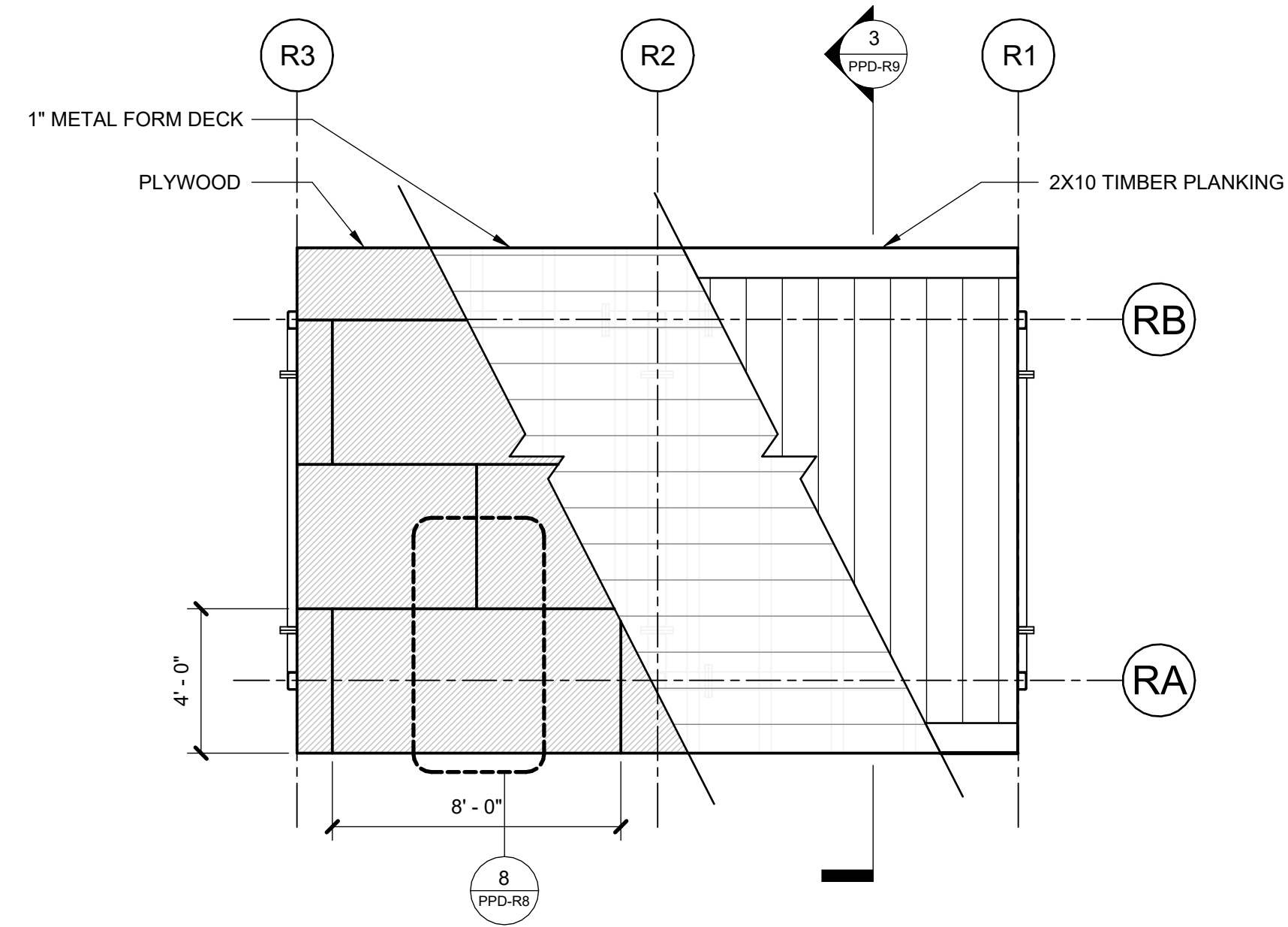
3 PART PLAN - DECK TYPE D3 1/4" = 1'-0"
