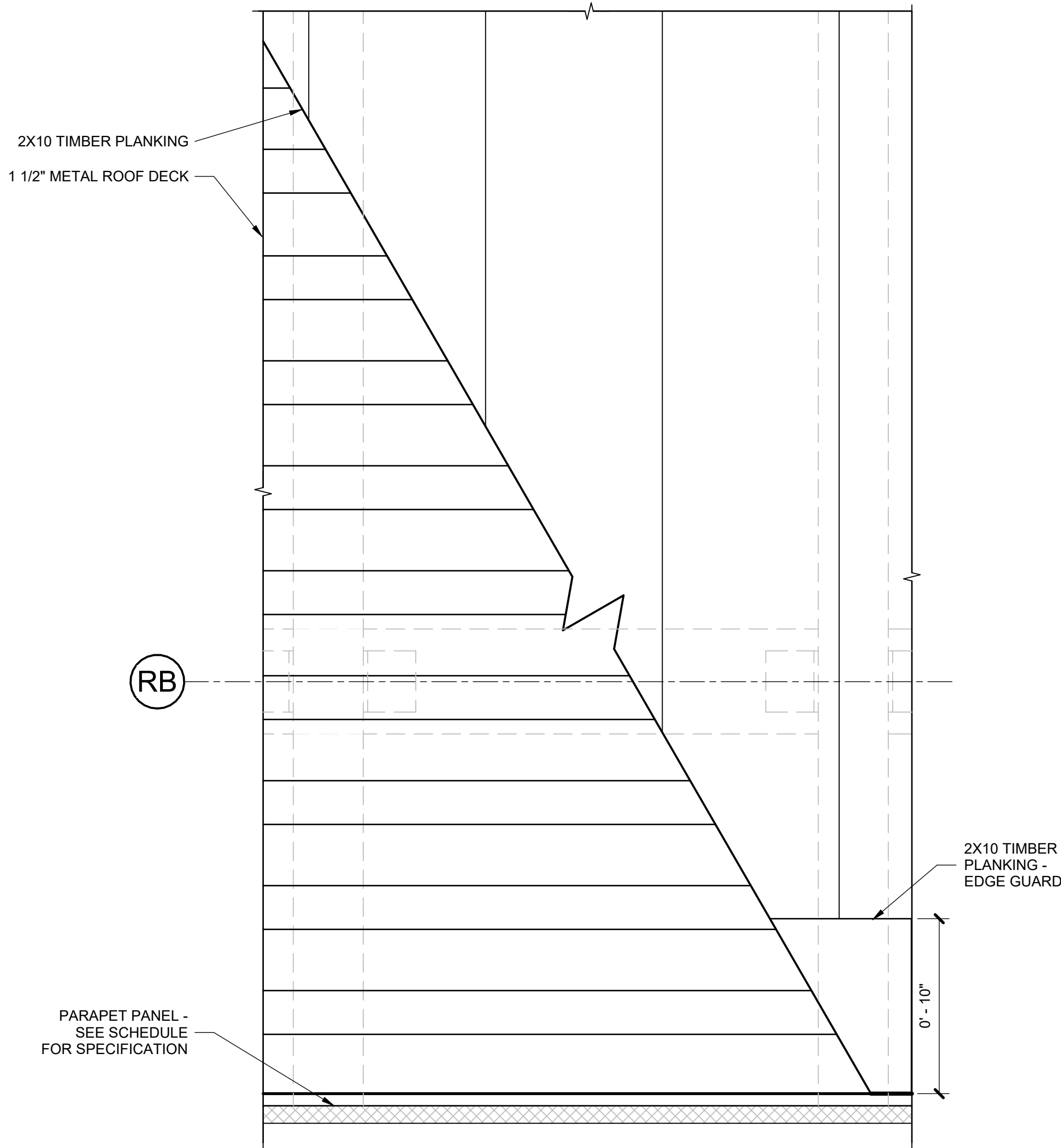
5 PLAN DETAIL - DECK TYPE D1 2" = 1'-0"
