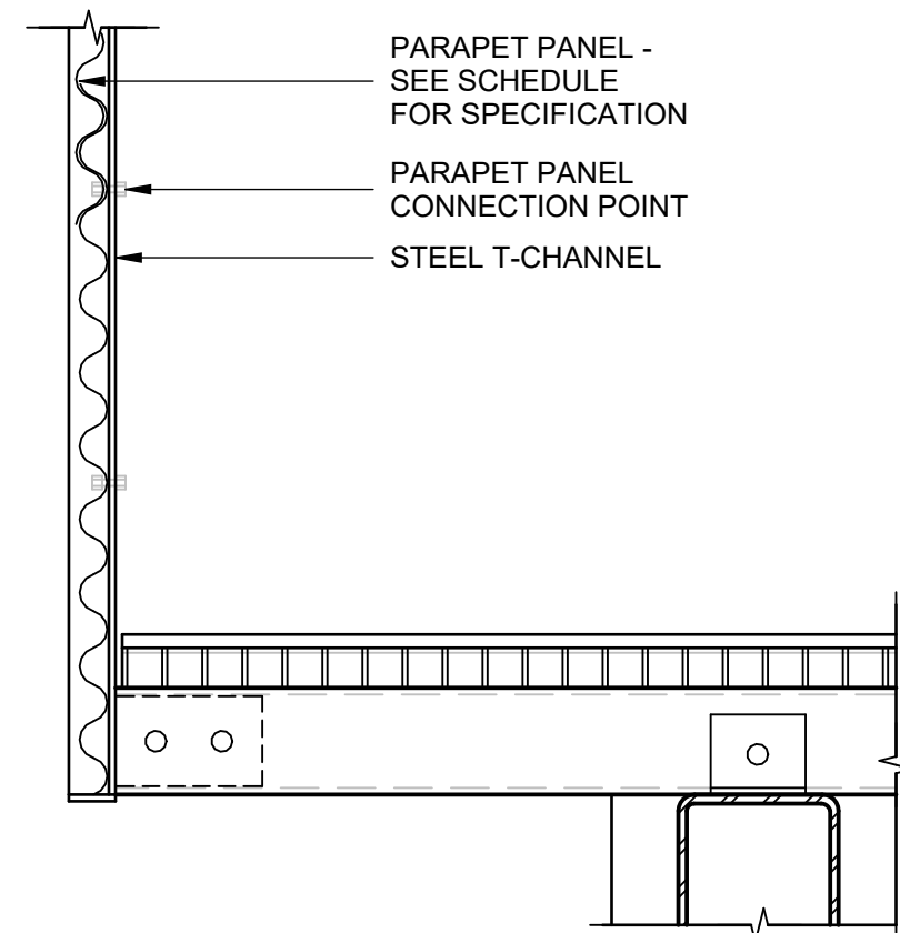
6 SECTION DETAIL 1 1/2" = 1'-0"
