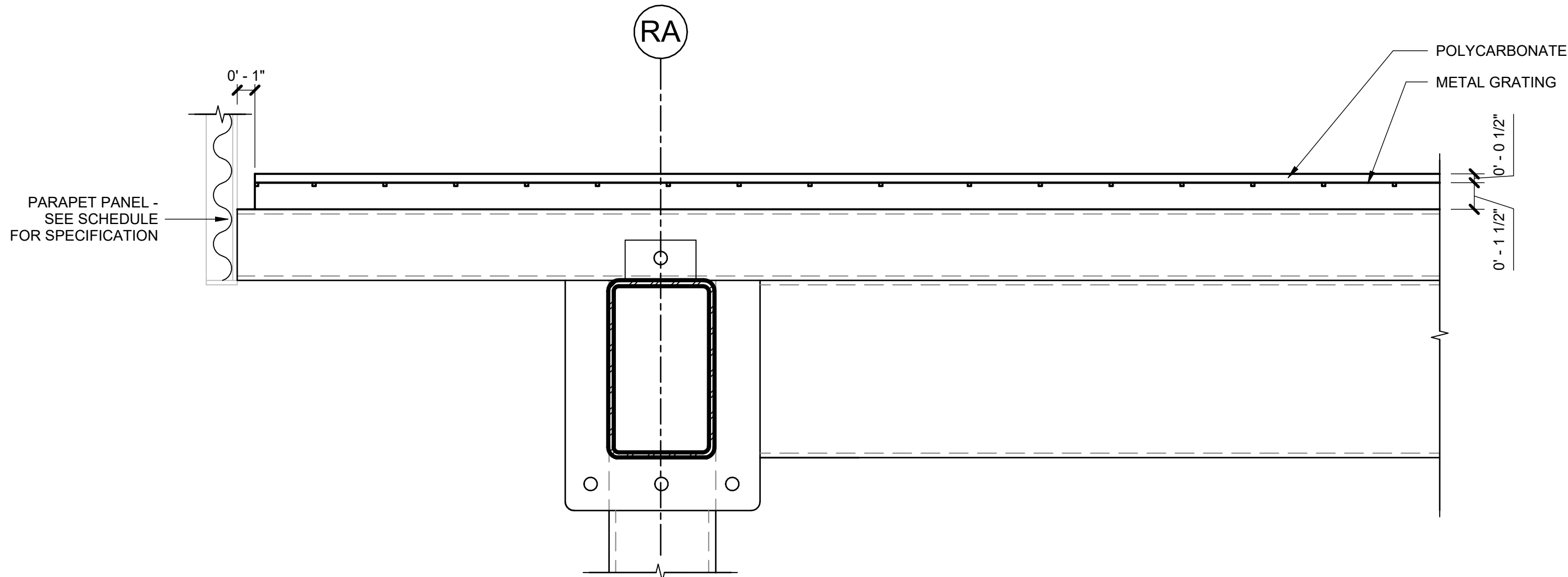
2 SECTION DETAIL - DECK TYPE D2 2" = 1'-0"
