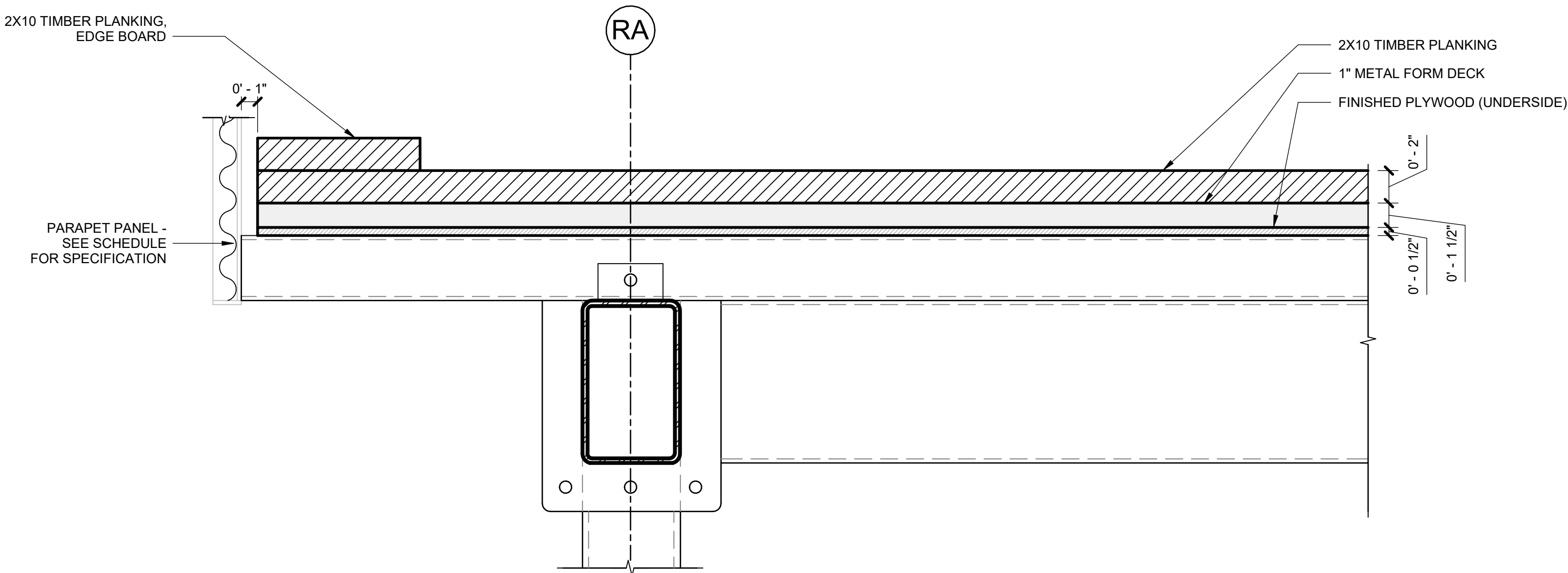
3 SECTION DETAIL - DETAIL D3 2" = 1'-0"
