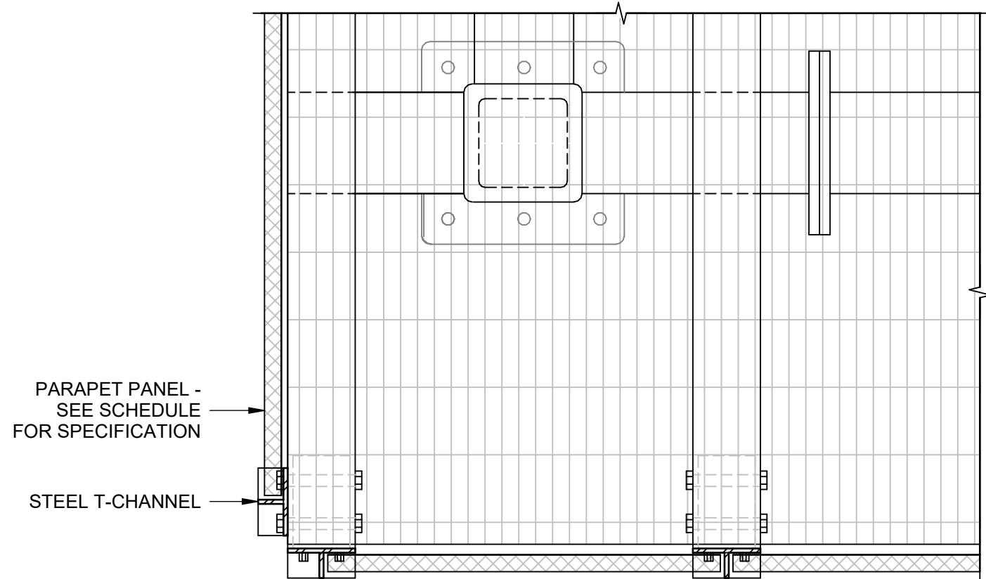
3 PLAN DETAIL - CORNER 1 1/2" = 1'-0"
