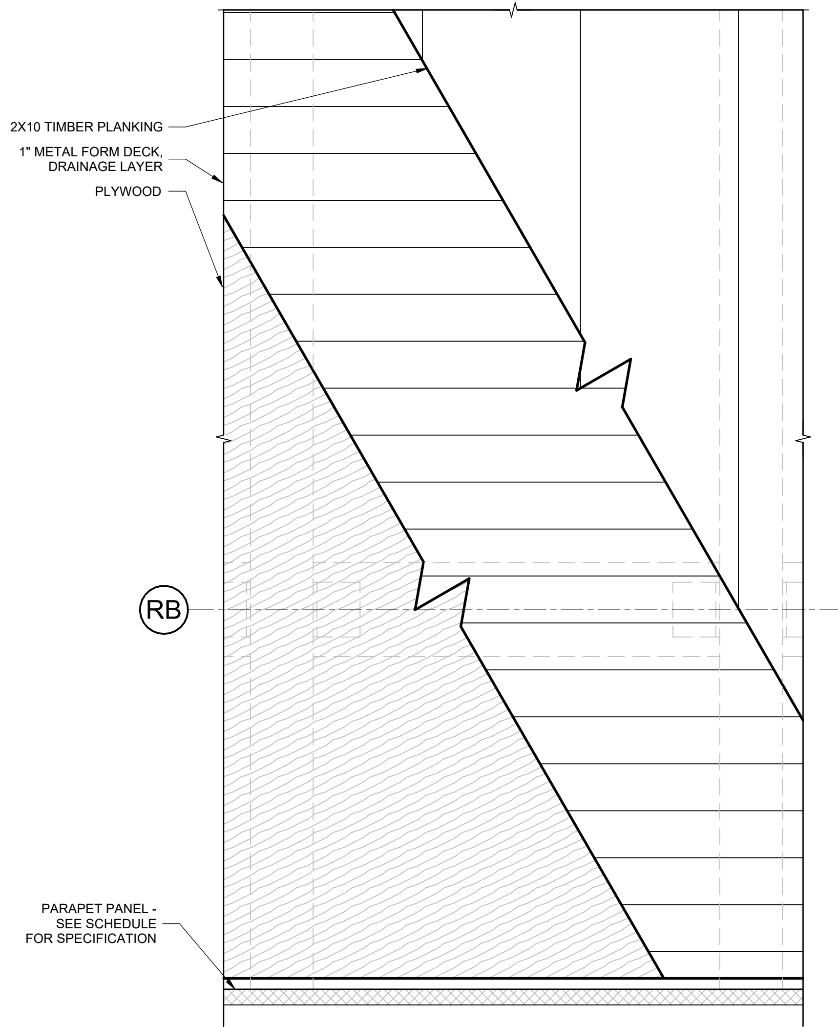
8 PLAN DETAIL - DECK TYPE D3 2" = 1'-0"
