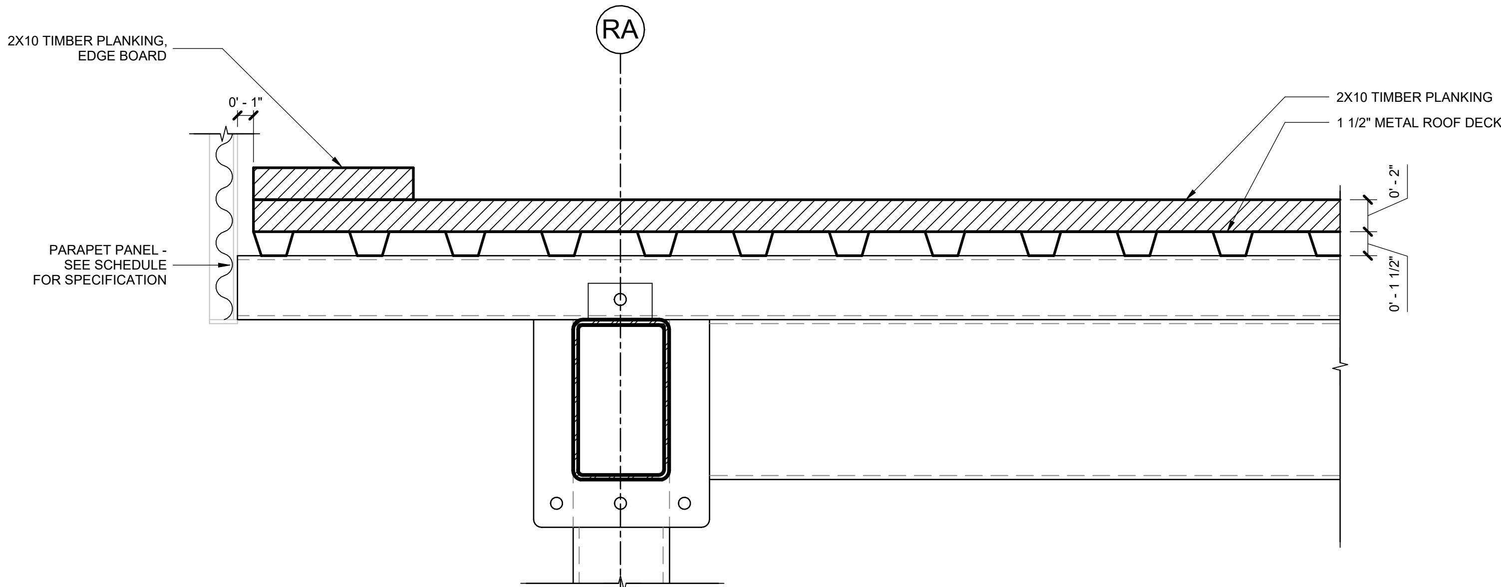
1 SECTION DETAIL - DECK TYPE D1 2" = 1'-0"
