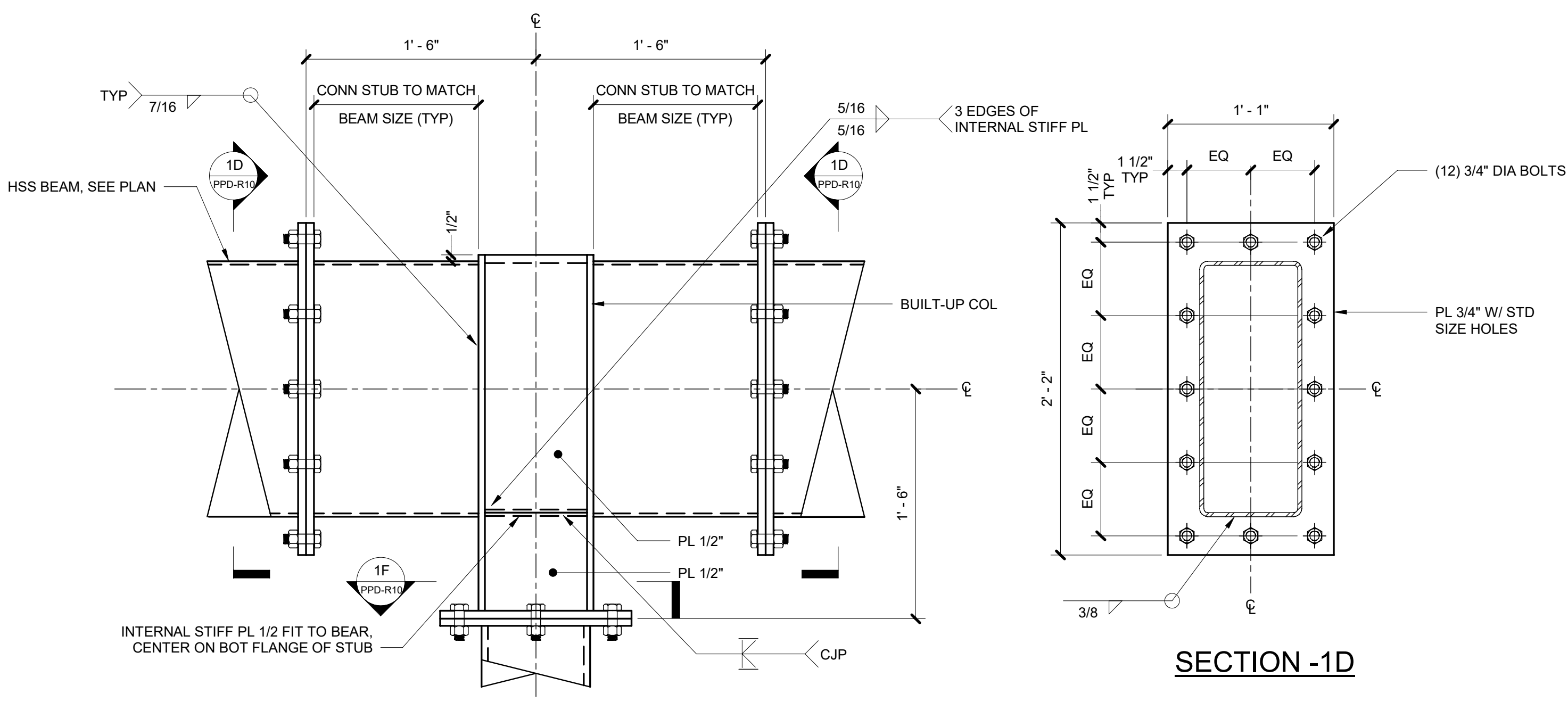
HSS20X8 BEAM/HSS8X8 COLUMN
