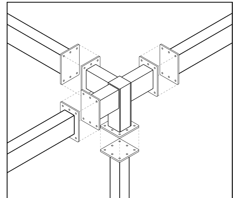
EXPLODED AXONOMETRIC - CONNECTION
