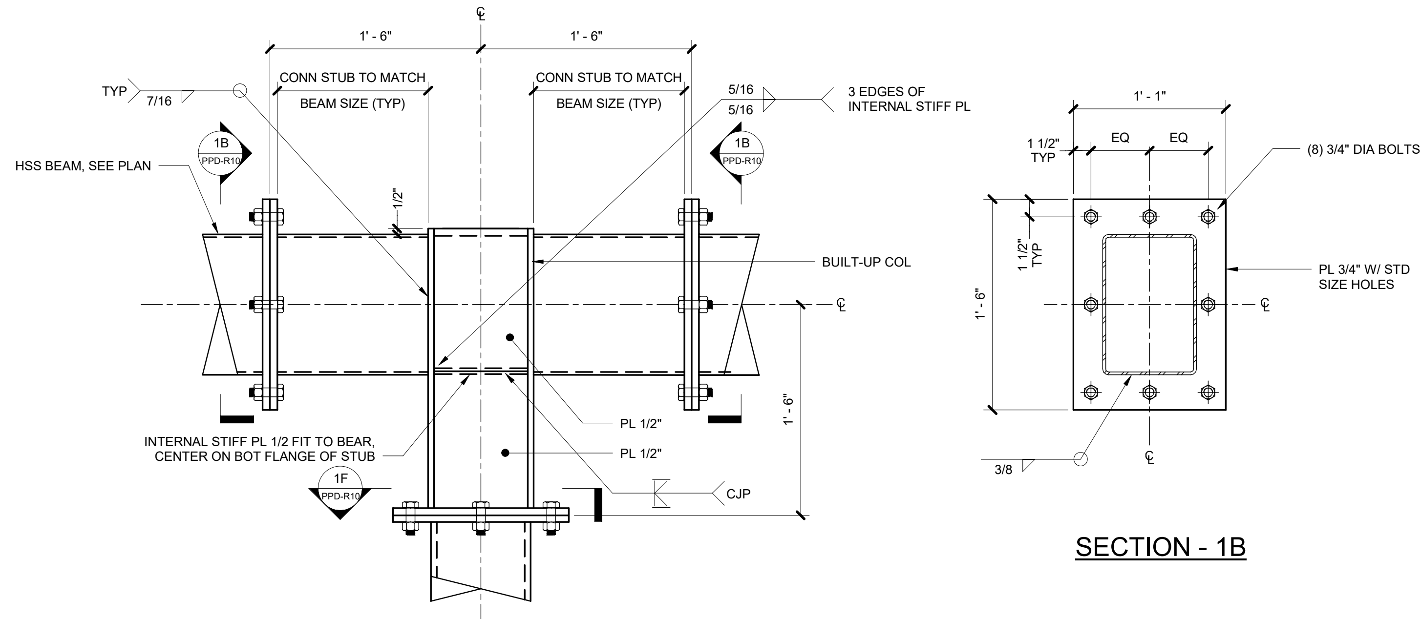
HSS12X8 BEAM/HSS8X8 COLUMN
