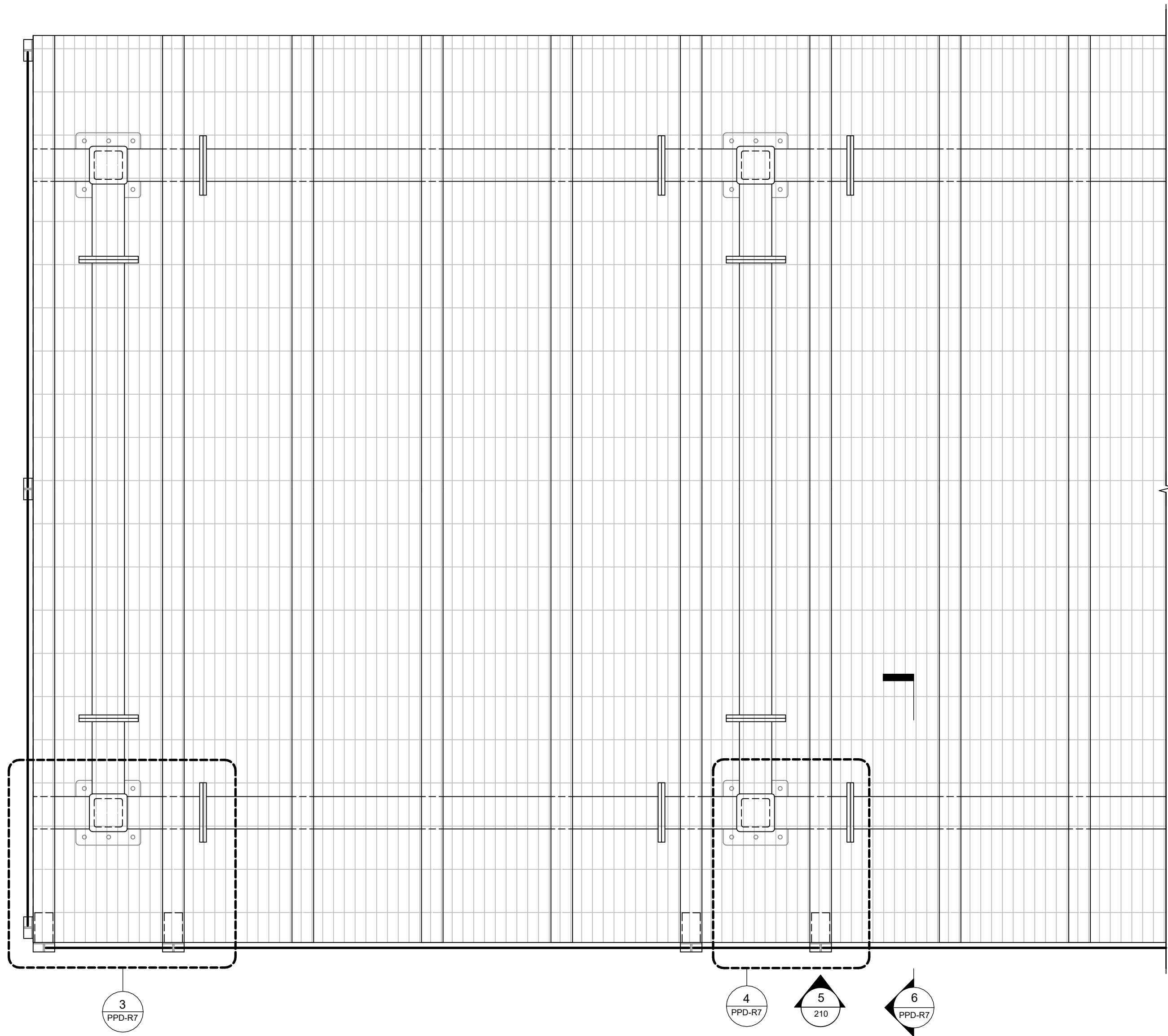
1 PART PLAN - END CONDITION 3/4" = 1'-0"
