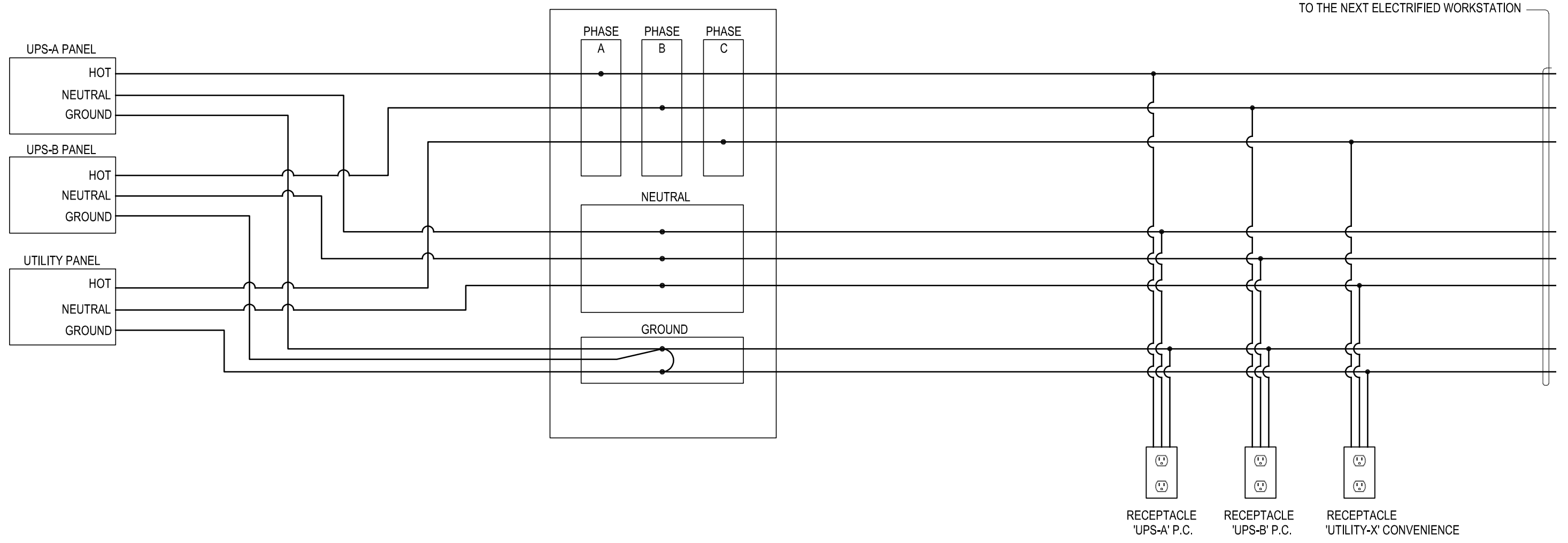
TYPICAL CIRCUITING FOR TRADING ELECTRIFIED FURNITURE SYSTEM (8 WIRE, 3 CIRCUIT SYSTEM)
