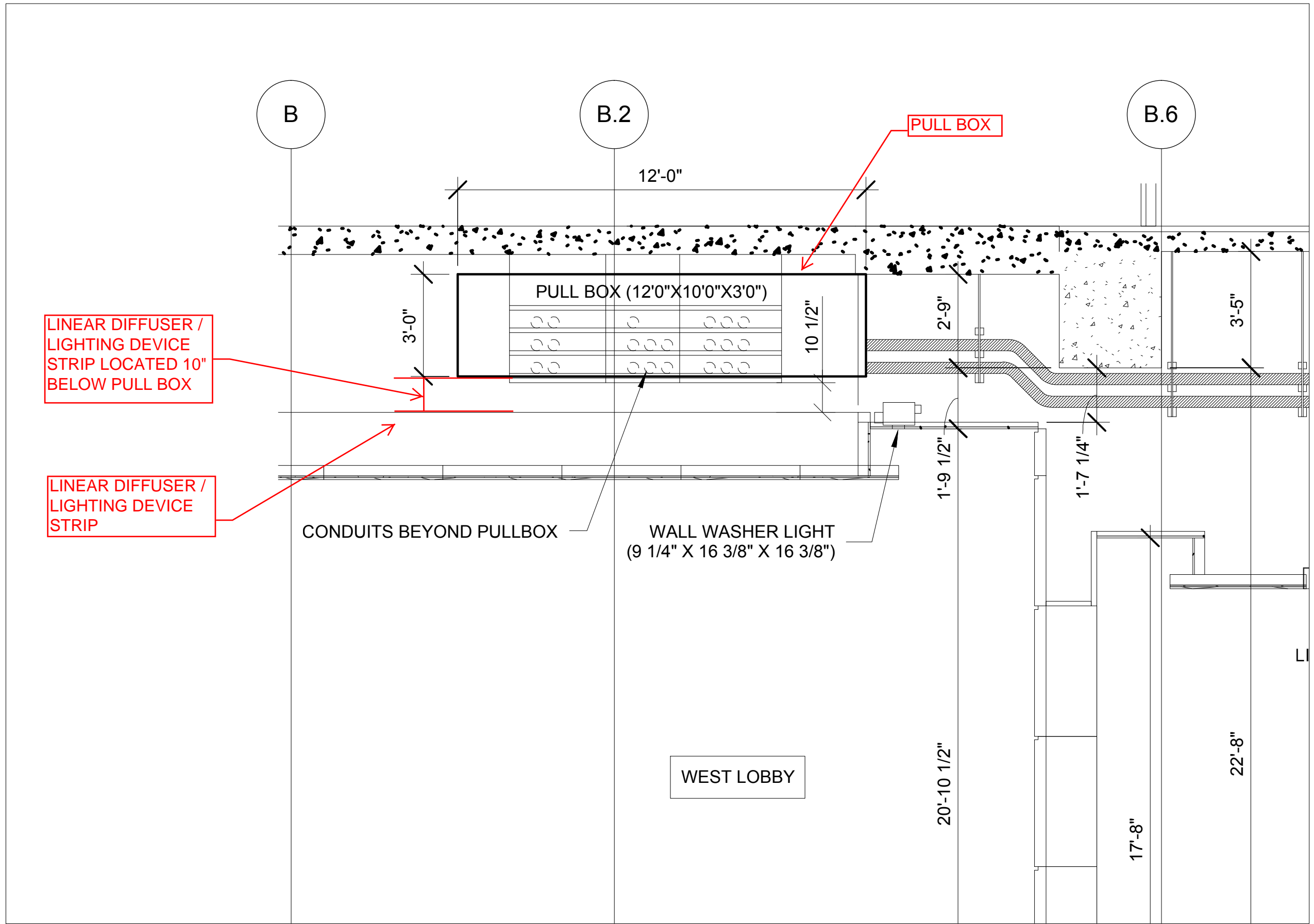
WEST LOBBY CEILING SECTION SKE-001-2
