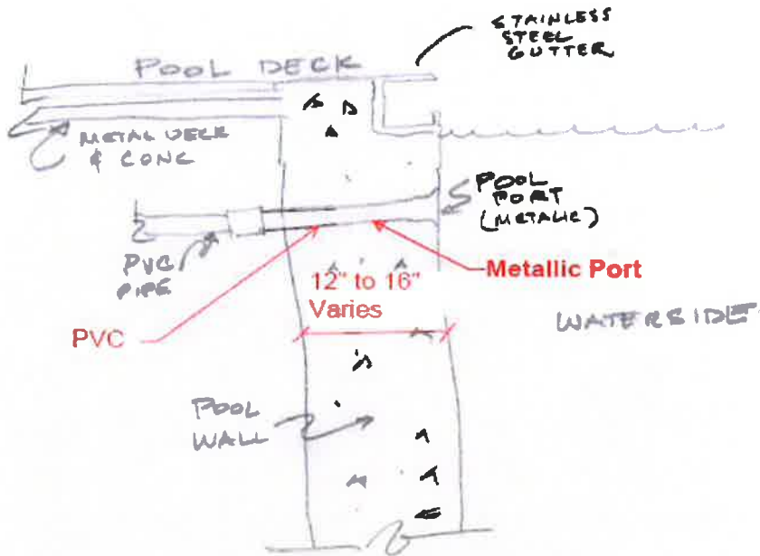
SECTION AT POOL PORT NTS
