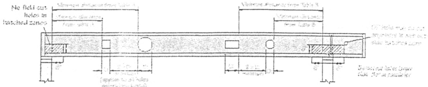
Figure 3. - Allowable Hole Size and Location for the TJI 110, TJI 210, TJI 230, TJI 360 and TJI 560 Joists
