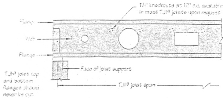
FIGURE 2. Allowable Hole Size and Location for the TJI/L45, TJI/L65, TJI/L90, TJI/H90, TJI/HD90 and TJI/HS90 Joists ONLY.
