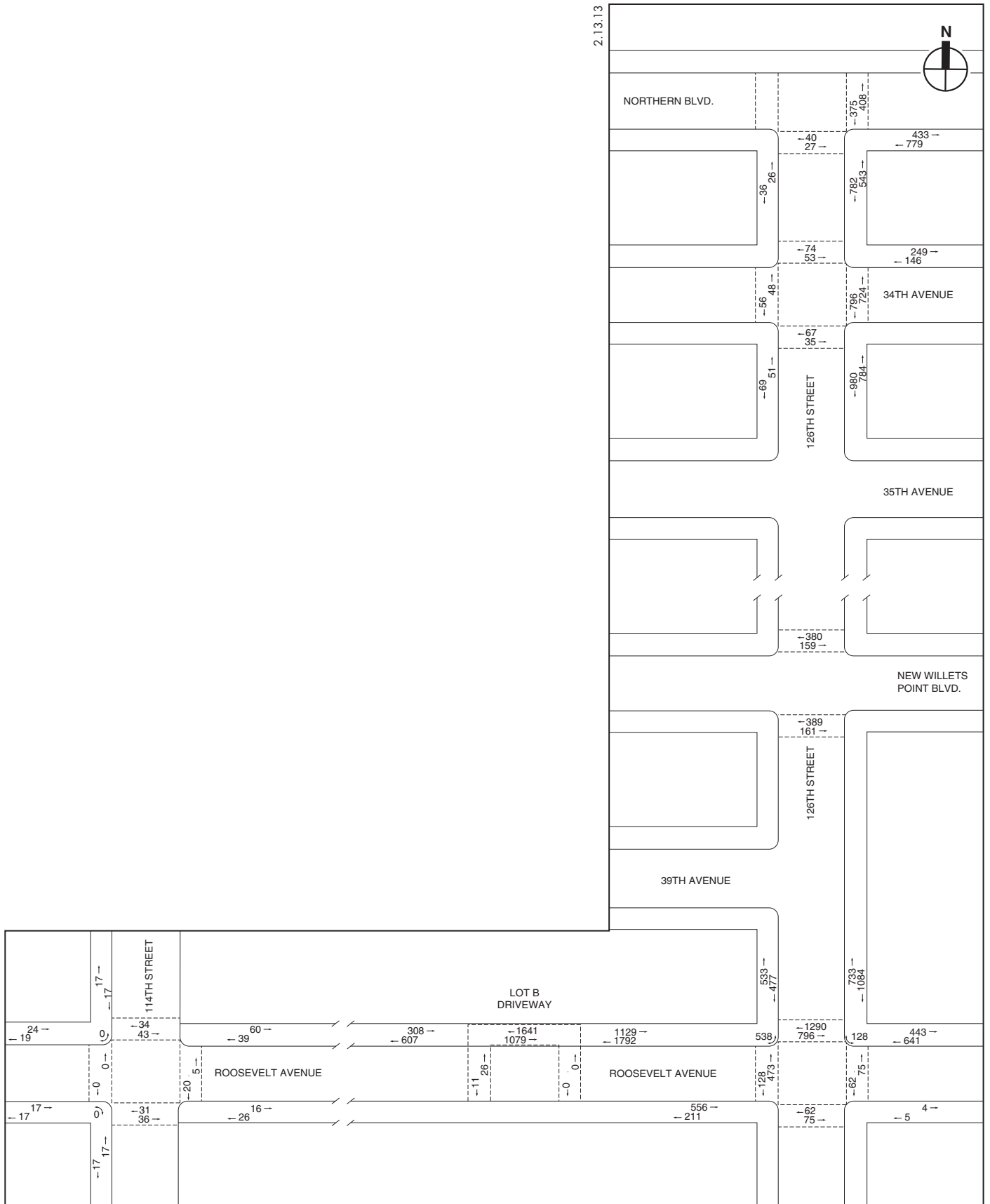
2032 With Action Pedestrian Increments Weekday AM Peak Hour
