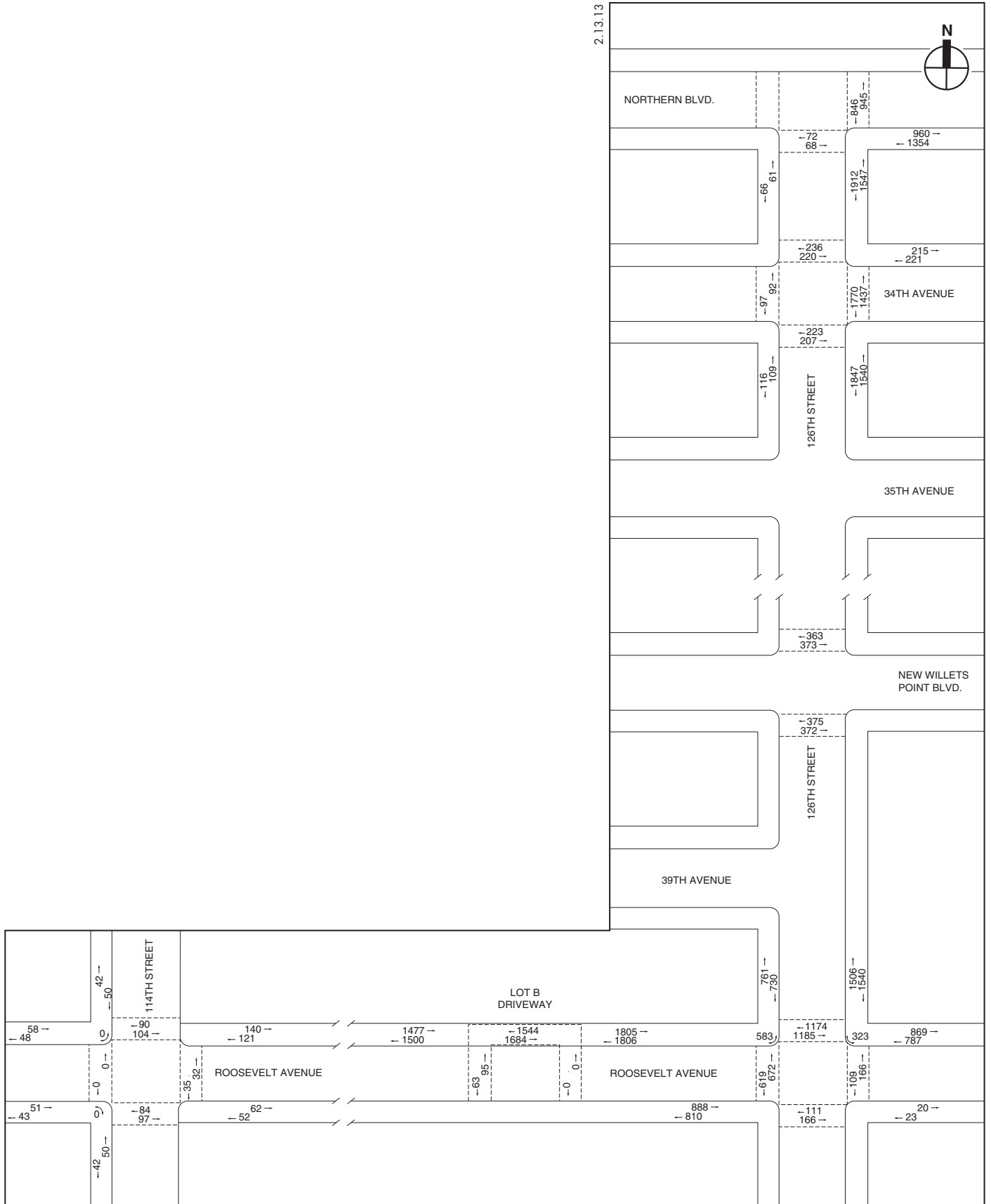
2032 With Action Pedestrian Increments Weekend Midday Non-Game Peak Hour
