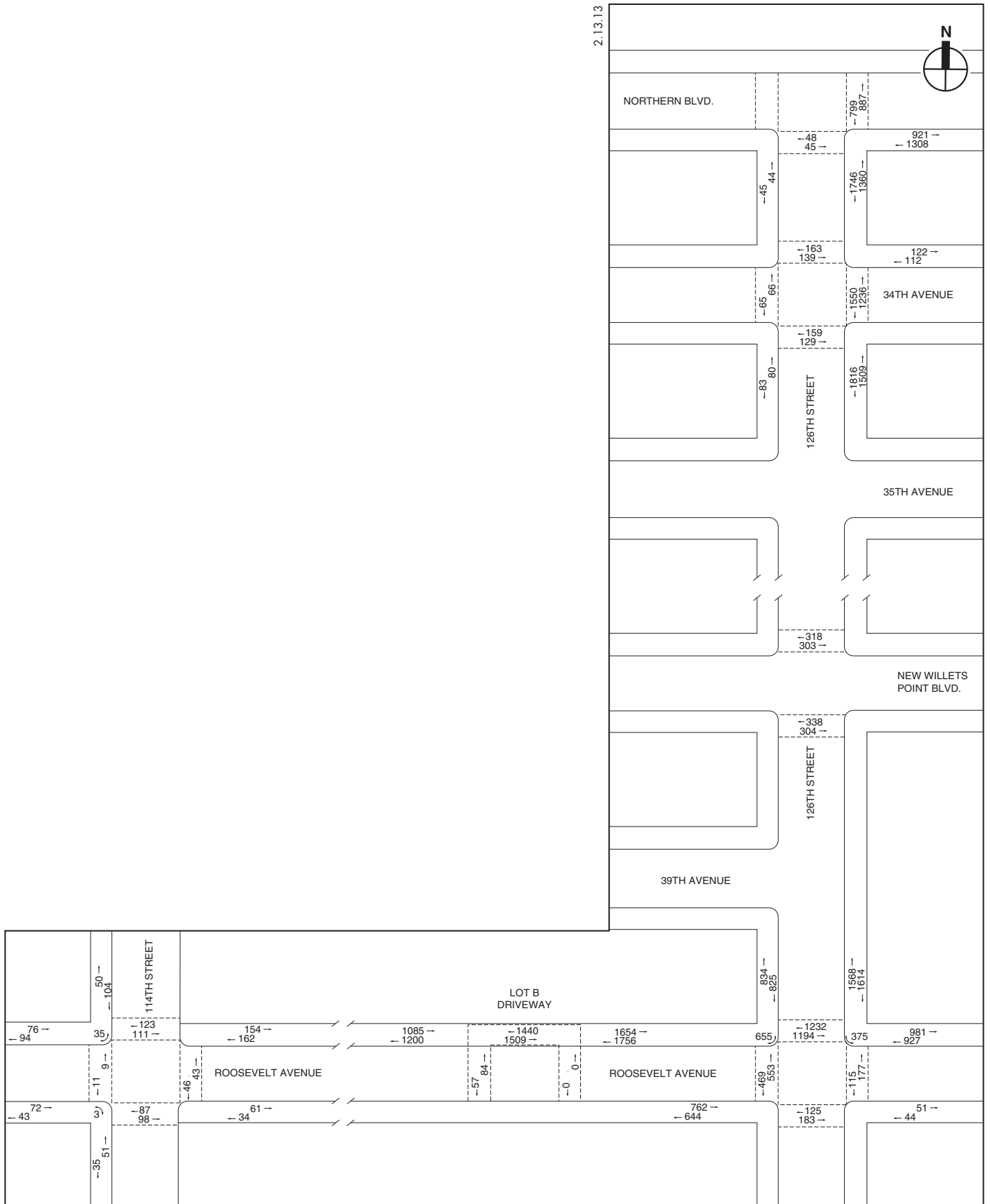
2032 With Action Pedestrian Volumes Weekday Midday Peak Hour
