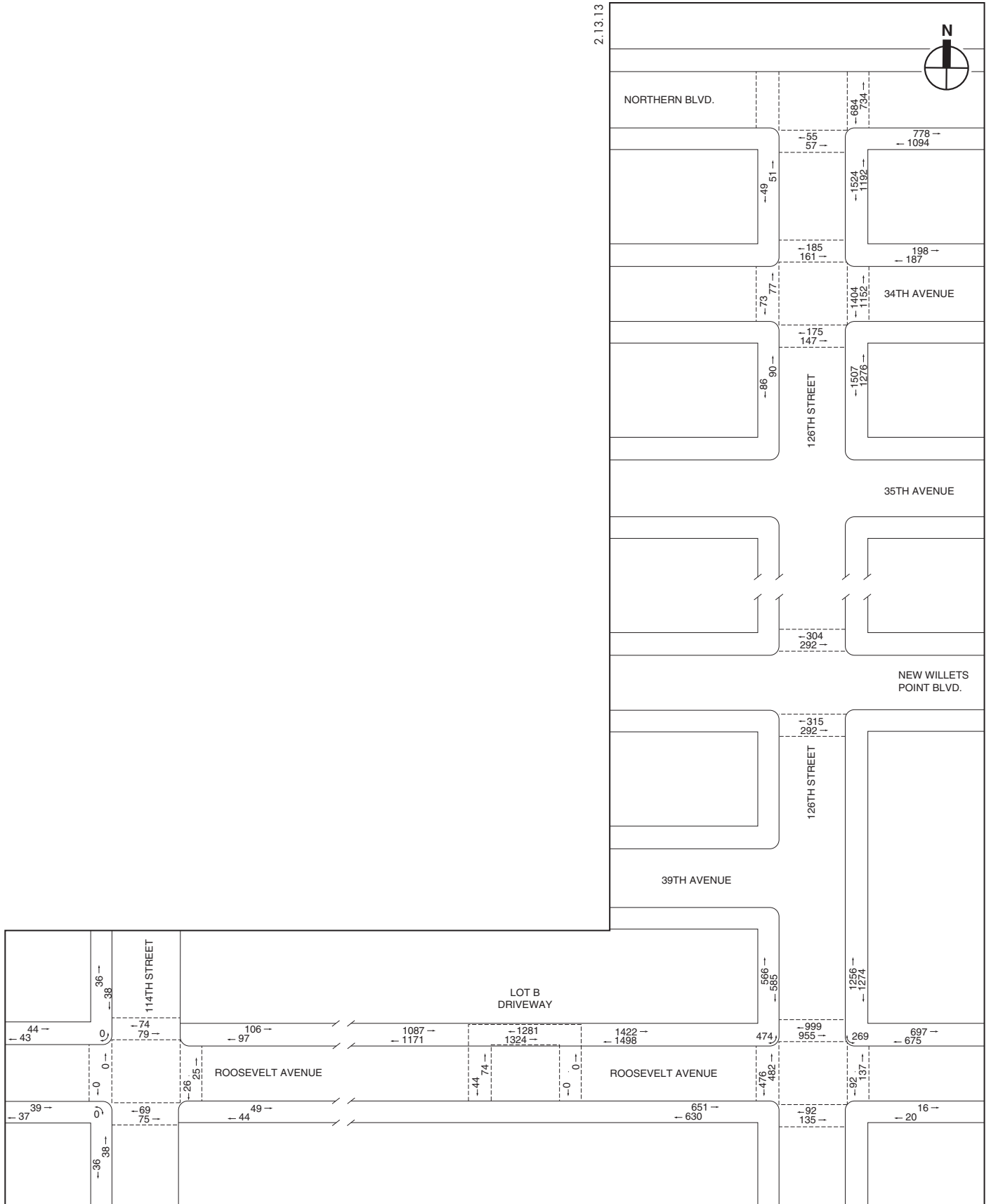
2032 With Action Pedestrian Increments Weekend Pre-Game Peak Hour
