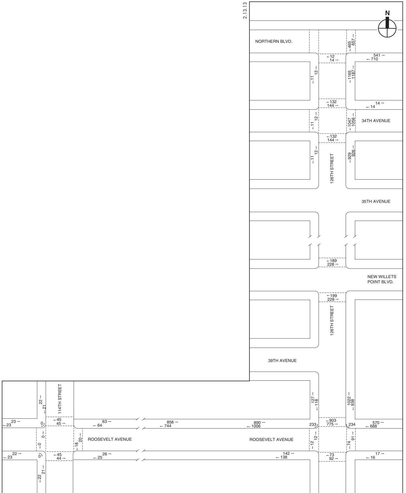
2028 With Action Pedestrian Increments Weekday PM Peak Hour
