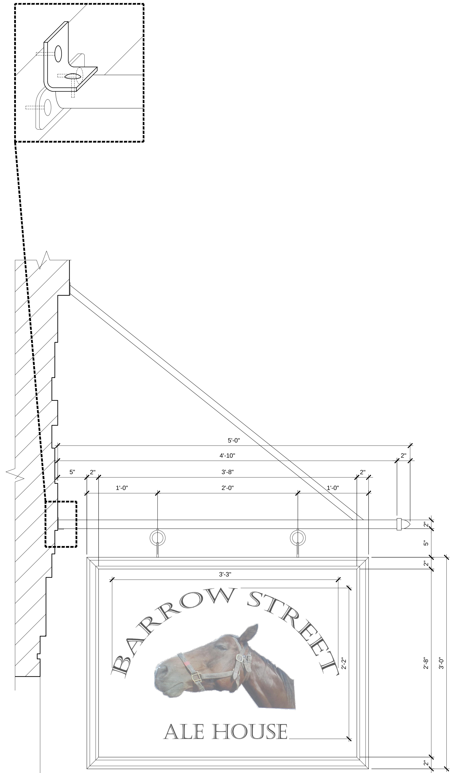
3 EXISTING SIGNAGE DETAILS A-101 SCALE: 1 1/2"=1'-0"
