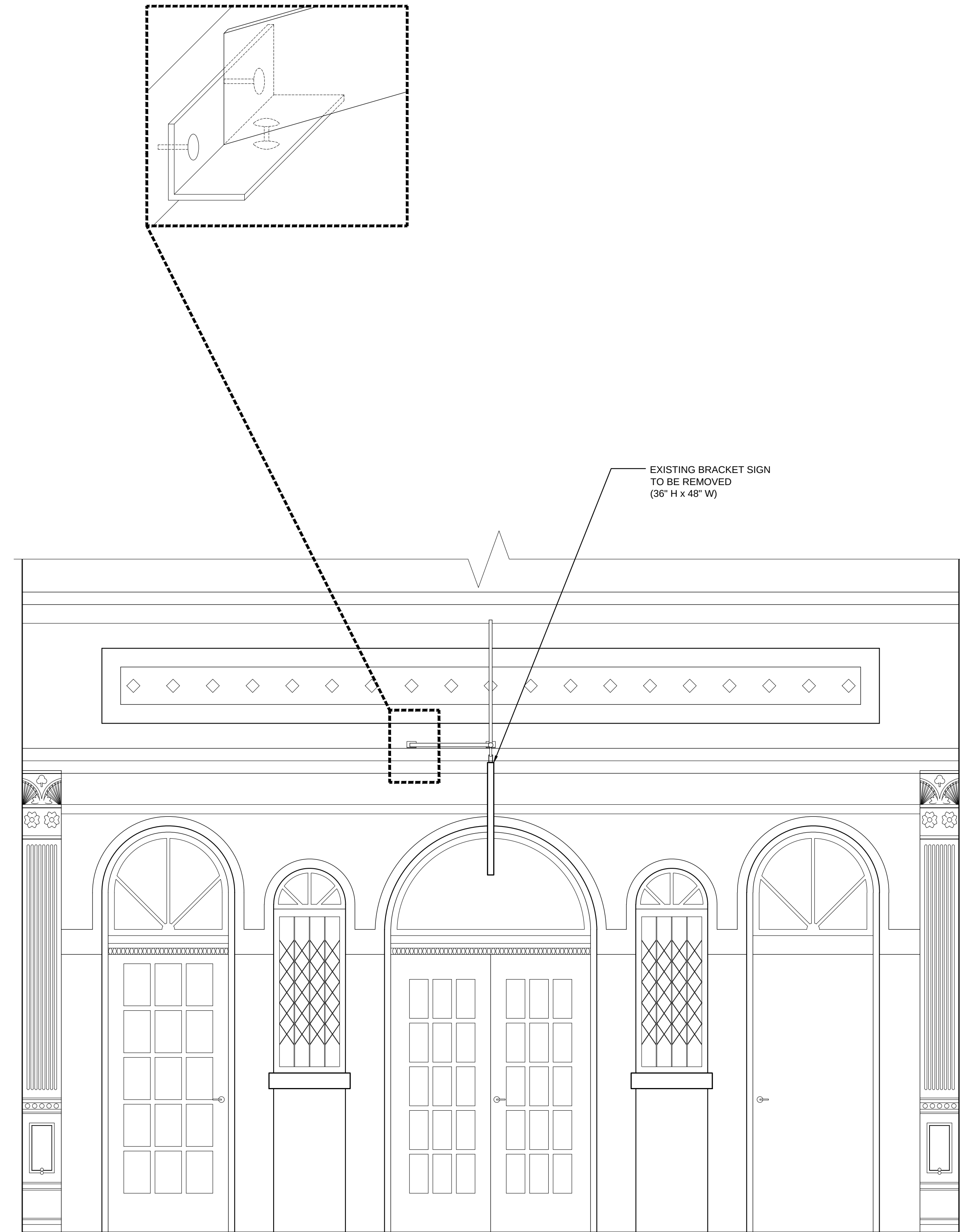
1 EXISTING STREET FACADE A-101 SCALE: 1/2"=1'-0"
