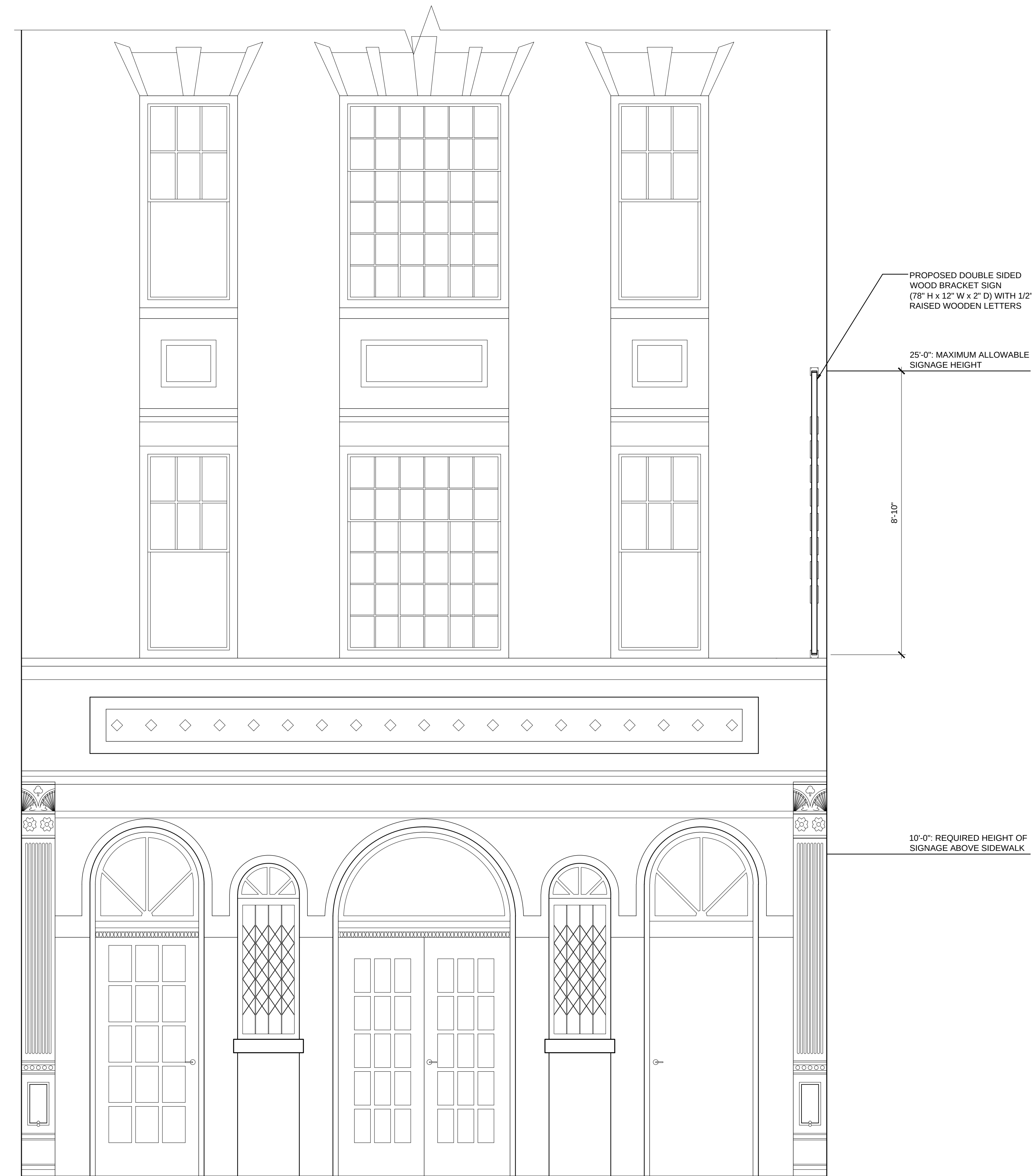
1 PROPOSED STREET FACADE A-102 SCALE: 1/2"=1'-0"
