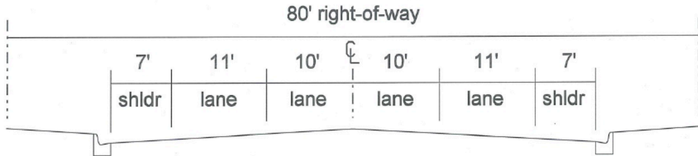
Water Street existing typical section
