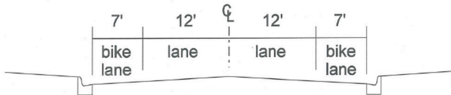
Shoreline Blvd proposed typical section
