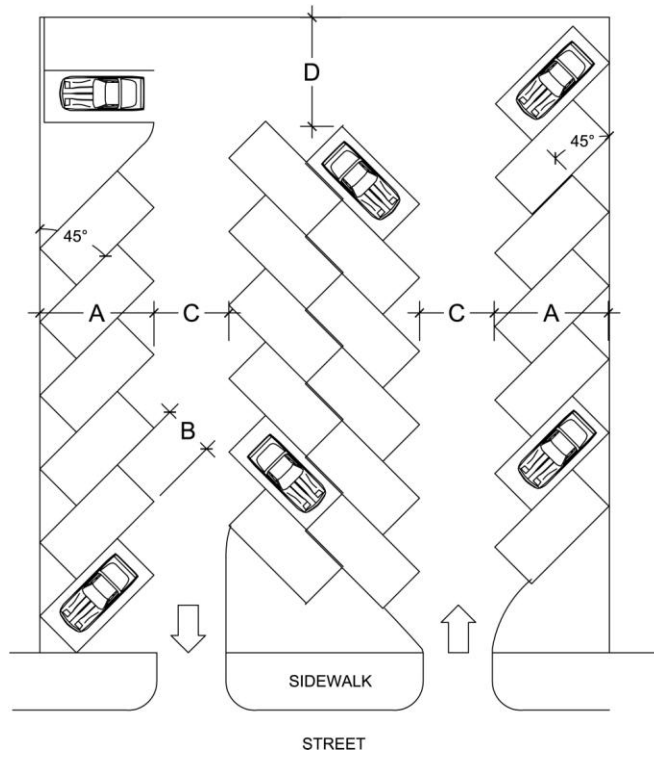
45 Degree Parking Layout
