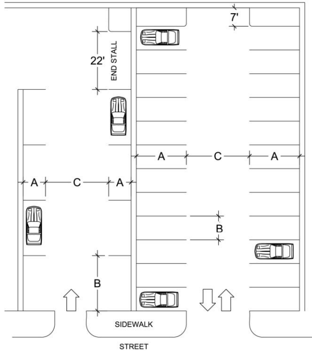
Parallel Parking/Dead-End Parking
