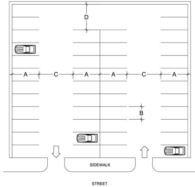
90 Degree Parking Layout
