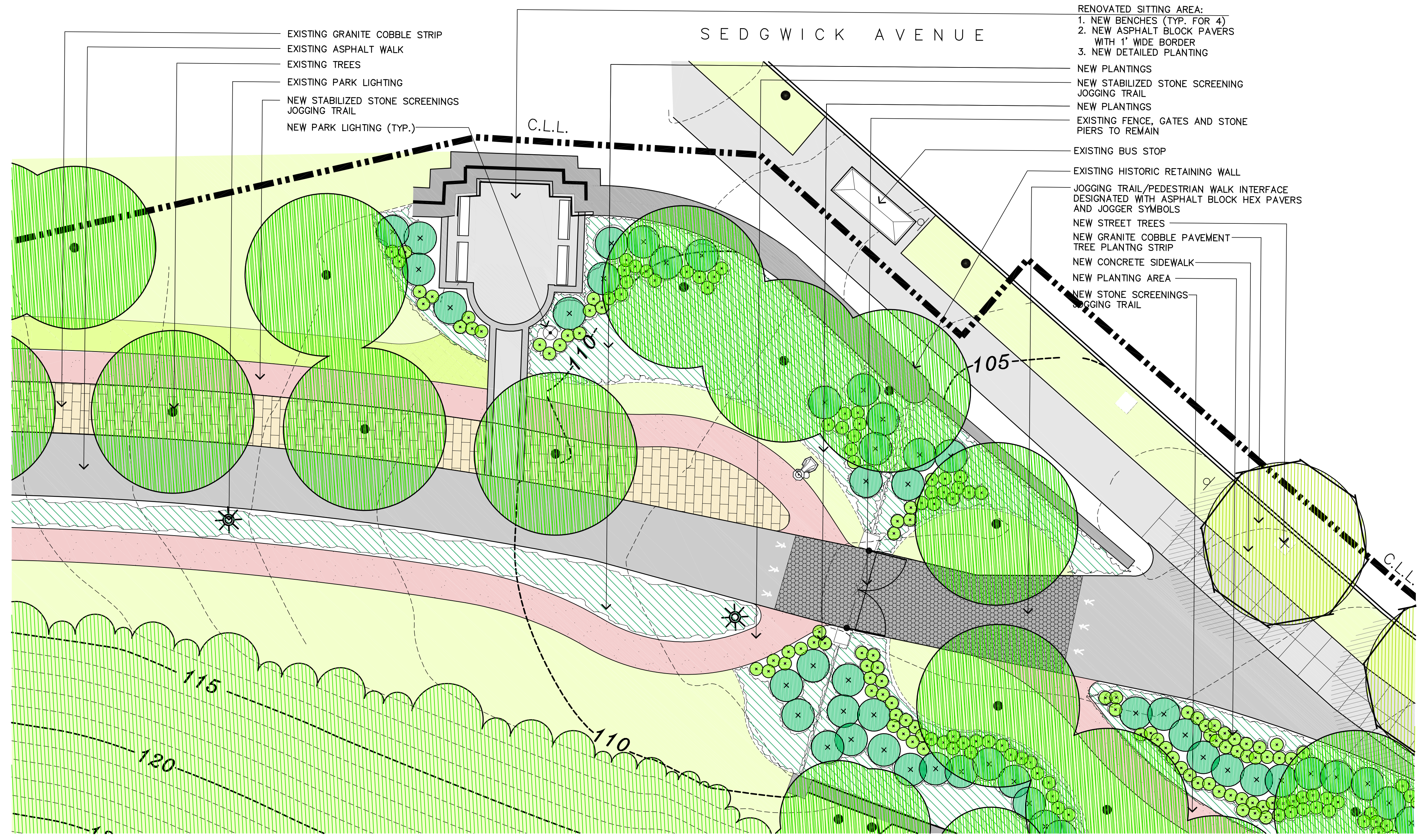
DETAIL PLAN 'D'- ENLARGEMENT PLAN AT FORT INDEPENDENCE PARK SCALE: 1" = 10'-0"
