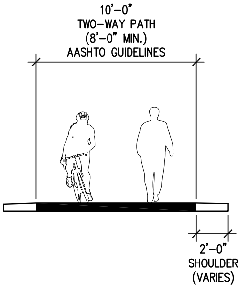
Figure 1.6: Minimum Trail Width
