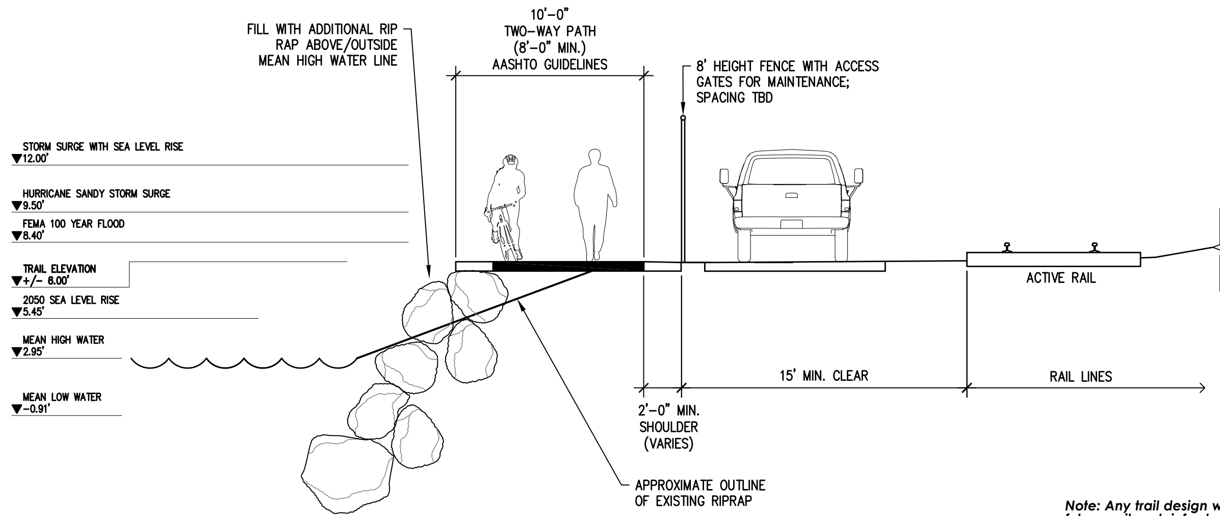
FIGURE 2.4: TYPE 2 TRAIL- BUILT-UP RIP-RAP
