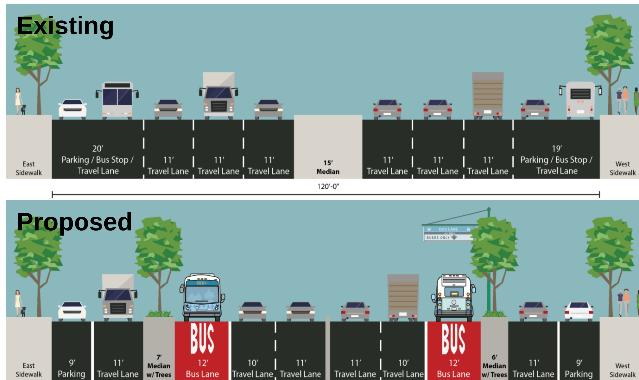
Typical 120' right-of-way
