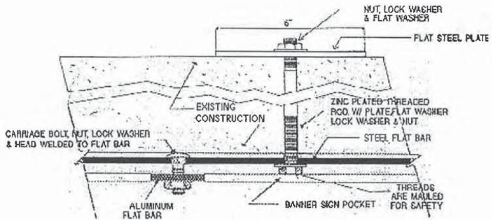
DETAIL A-2 THRU BOLT INSTALLATION PLAN ( AT EACH END )
