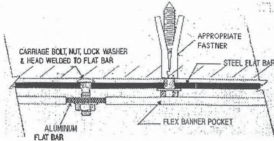
DETAIL A-1 WALL ANCHOR INSTALLATION PLAN
