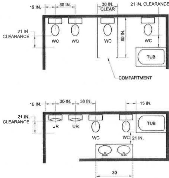
[FIGURE 405.3.1 FIXTURE CLEARANCE] For SI: 1 inch = 25.4 mm
